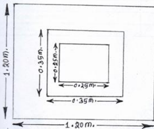
CROSS-SECTION OF COLUMN
