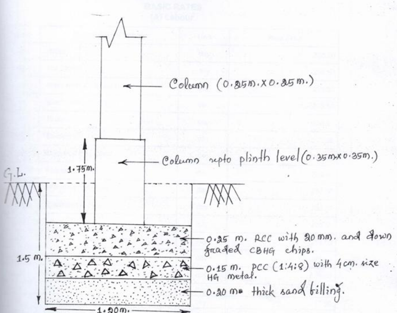
CROSS-SECTION OF COLUMN
