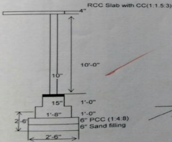
CS OF FOUNDATION FOOTING
