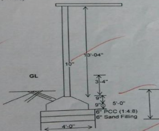
CS OF COLUMN FOUNDATION
