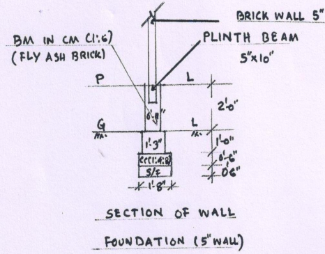
CONSTRUCTION OF MPA OFFICE BUILDING (OPELIP) AT PBDA, KHUNTAGAON UNDER LAHUNIPARA BLOCK.
